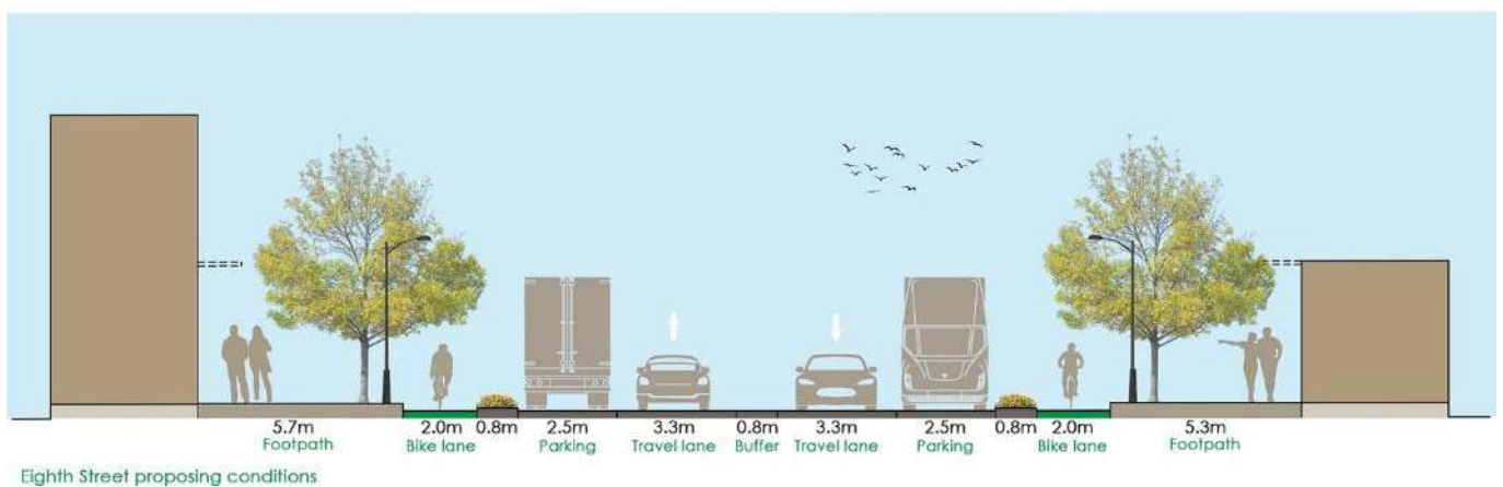
Figure 20 Option B - Existing and proposed cross-section (Eighth Street)
