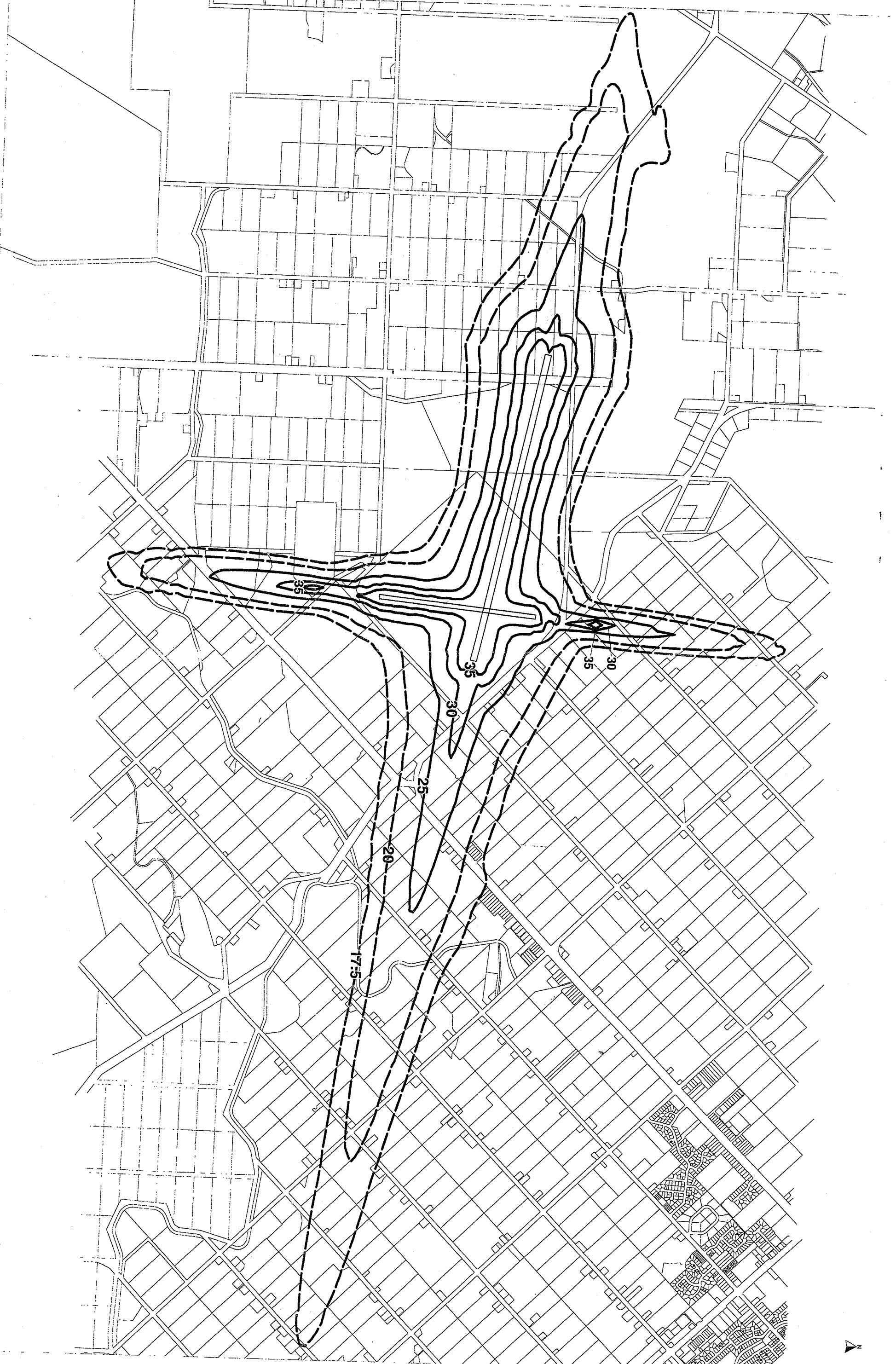
Mildura Airport - Year 2015 ANEF Noise Contours
